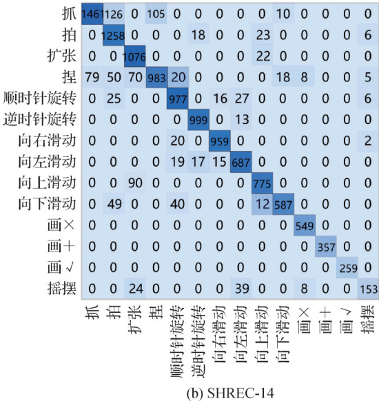
图 7 模型在 DHG-14 和 SHREC-14 数据集的混淆矩阵 Fig. 7 Confusion matrix of the model on DHG-14 dataset and SHREC-14 dataset ((a) DHG-14; (b) SHREC-14)
