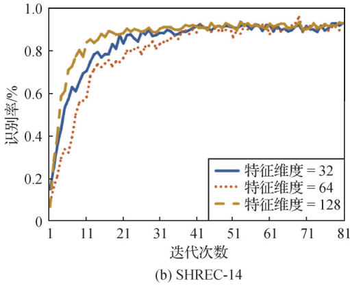
图 6 模型对 DHG-14 和 SHREC-14 不同维度的识别率 Fig. 6 Recognition rate of the model for different dimensions of DHG-14 and SHREC-14 (a) DHG-14; (b) SHREC-14)
