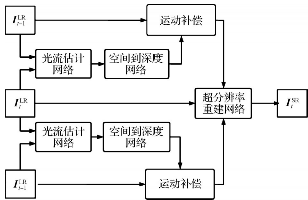
图9 SOFVSR的网络结构(Wang等,2018a) Fig. 9 The network architecture of SOFVSR (Wang et al. ,2018a)
