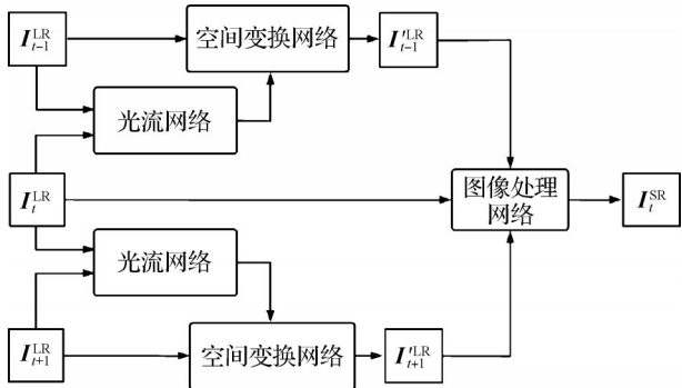
图10 ToFlow的网络结构(Xue等,2019) Fig. 10 The network architecture of ToFlow(Xue et al. ,2019)
