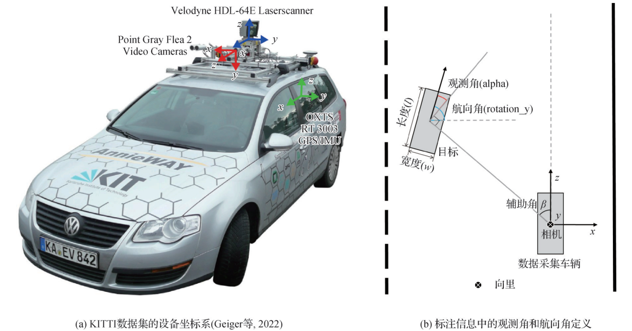
图2 KITTI数据集坐标系、目标的观测角和航向角定义 Fig. 2 Definitions of coordinate system, alpha and rotation_y of KITTI dataset ((a) equipment coordinate system of KITTI dataset (Geiger et al., 2022); (b) definitions of alpha and rotation_y)
