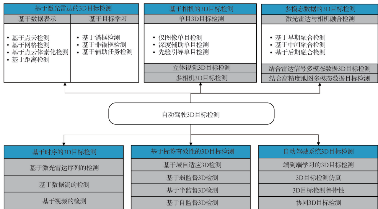
图1 用于自动驾驶3D目标检测的层次结构分类法(Mao等,2022) Fig. 1 A hierarchical taxonomy for 3D object detection in autonomous driving (Mao et al. , 2022)
