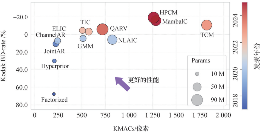
图 7 国内外方法性能复杂度对比 Fig. 7 Performance and complexity comparison of domestic and international methods
