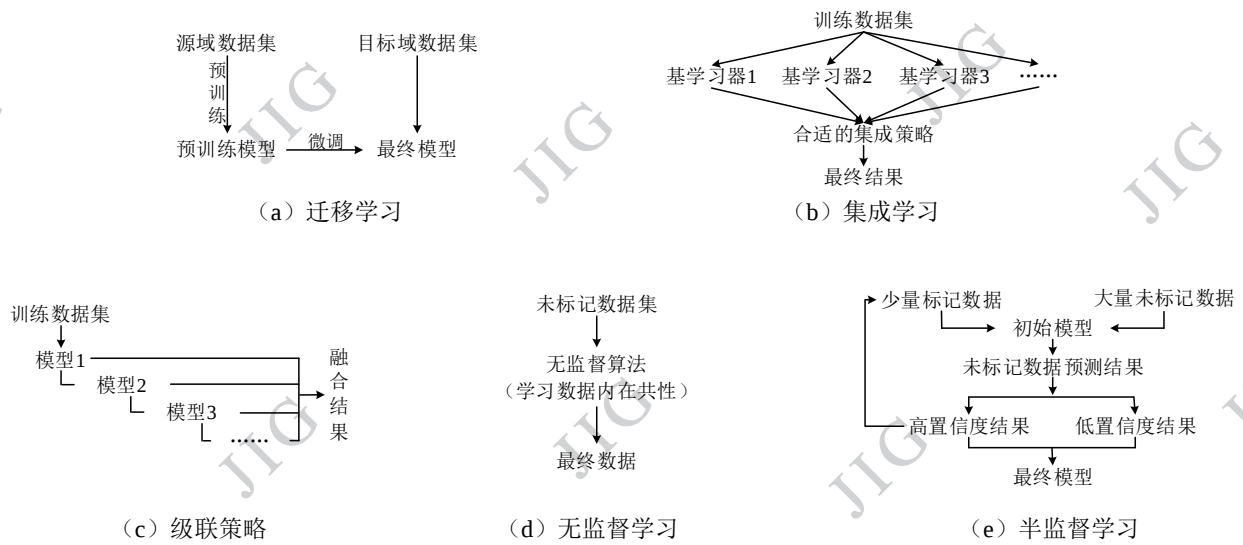
((a)transfer learning;(b)ensemble learning;(c)cascade strategy;(d)unsupervised learning;(e)semi-supervised learning)
