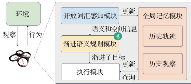
图6 CityNavAgent 工作流程 Fig. 6 The overall workflow of CityNavAgent
