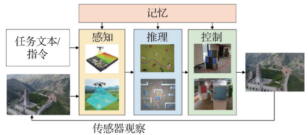
图3 无人机视觉语言导航认知闭环 Fig. 3 Cognitive closed-loop for UAV vision-language navigation
