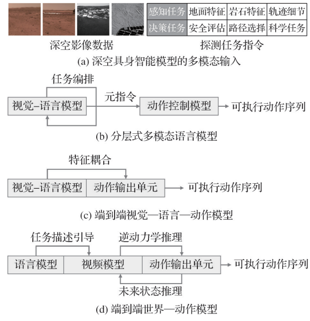
图2 具身智能模型概述 Fig. 2 Overview of embodied intelligence model ( (a) multimodal inputs for deep-space embodied intelligence model; (b) hierarchical multimodal language model; (c) end-to-end vision-language-action model; (d) end-to-end world-action model )
