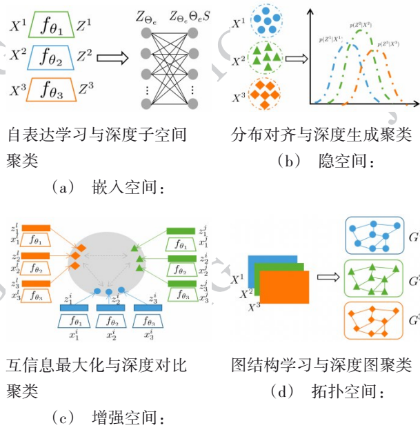
(a) embedding: self-expression & subspace clustering; (b) Latent: distribution alignment & generative clustering; (c) augmented: MI maximization & contrastive clustering; (d) topological: graph structure & graph clustering)
